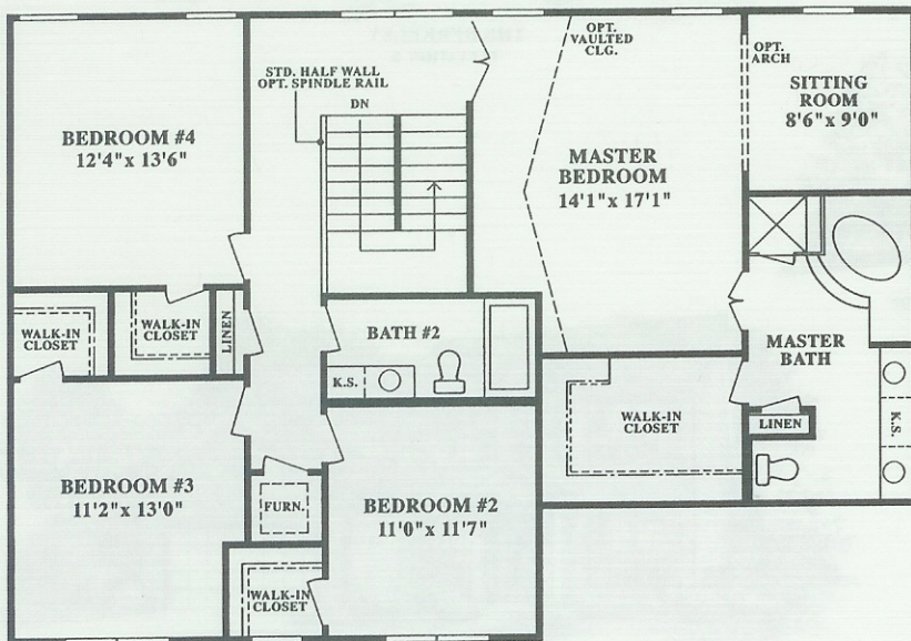
SECOND FLOOR PLAN THE BERKELEY
