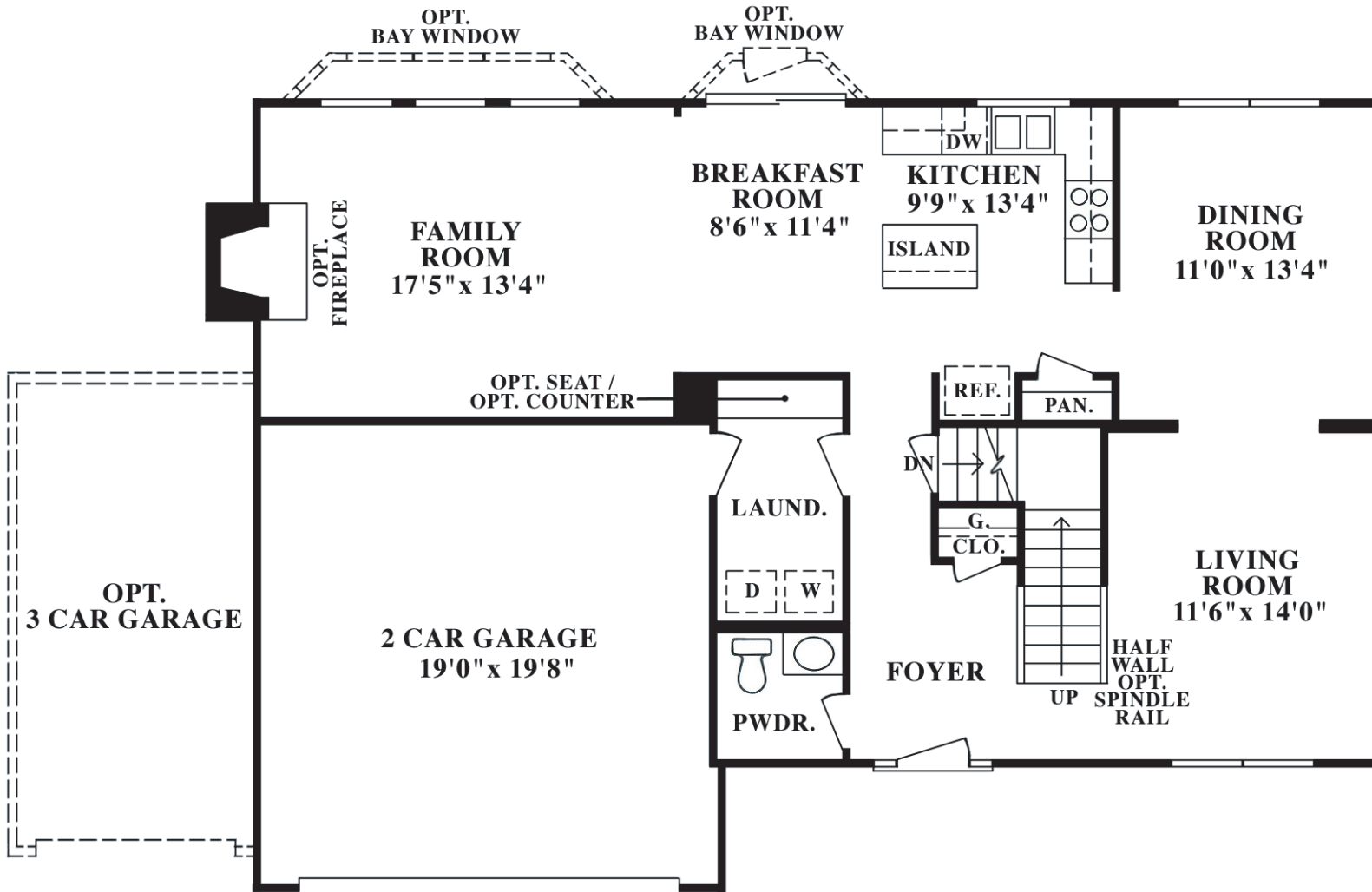
STANDARD FIRST FLOOR PLAN
