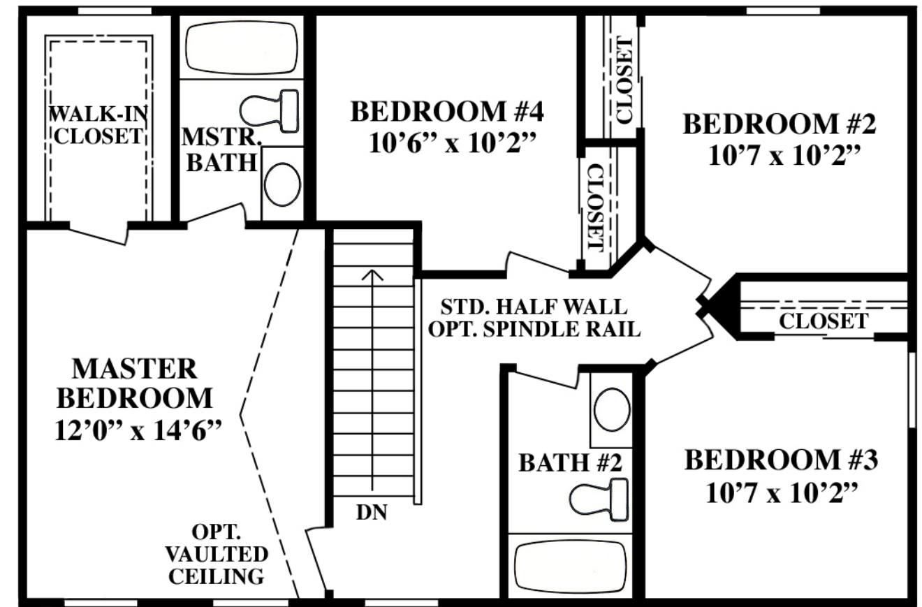
OPTIONAL 4 BEDROOM SECOND FLOOR PLAN
