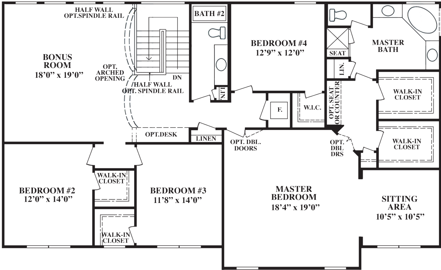
STANDARD SECOND FLOOR PLAN
